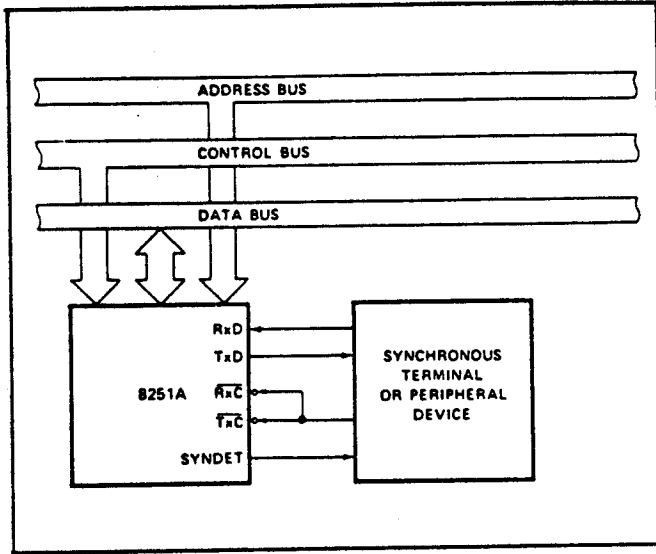
Figure 15. Synchronous Interface to Terminal or Peripheral Device
