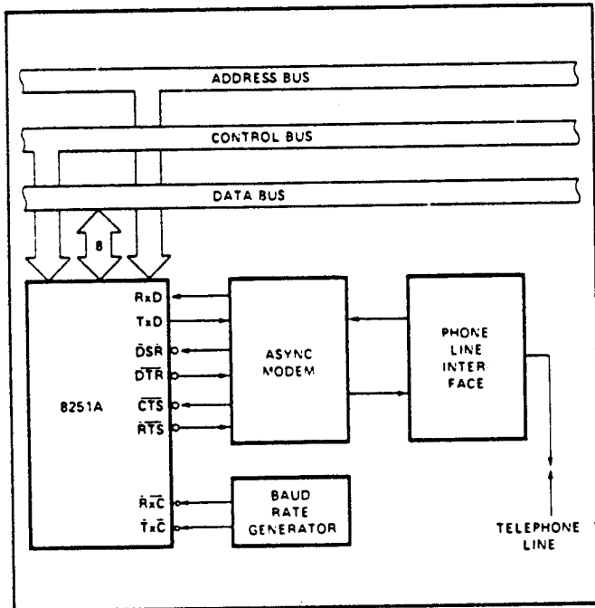
Figure 16. Asynchronous Interface to Telephone Lines
