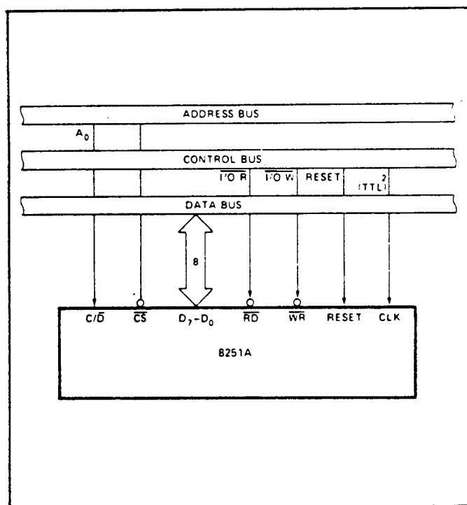
Figure 6. 8251A Interface to 8080 Standard System Bus
