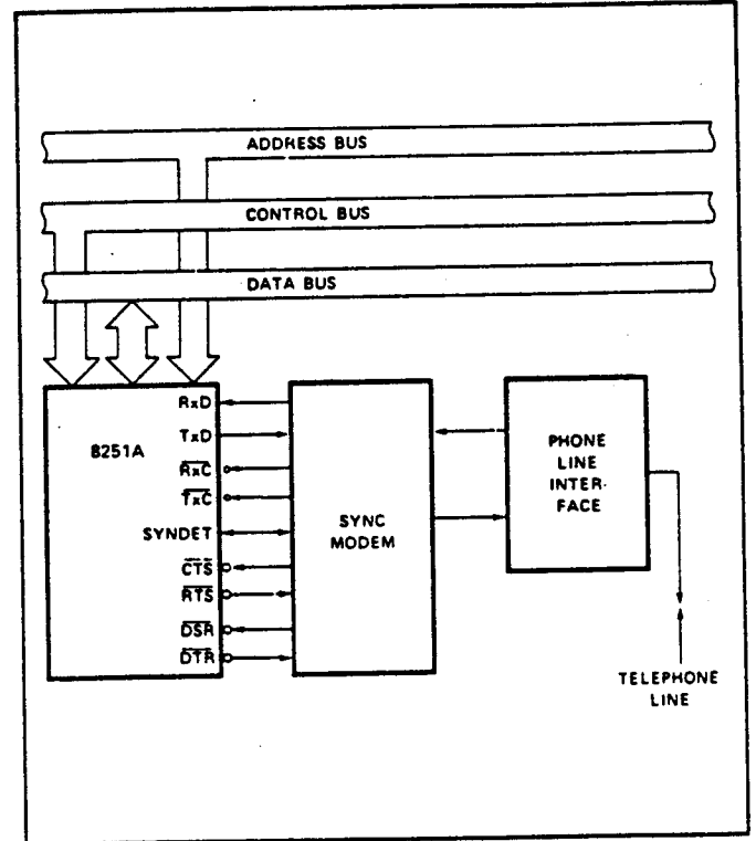
Figure 17. Synchronous Interface to Telephone Lines
